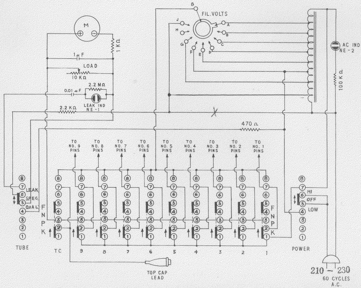
SCHEMATIC DIAGRAM
